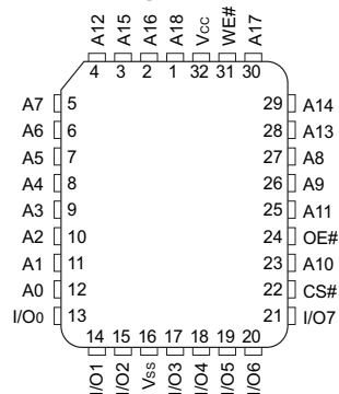
32 CLCC Top View
