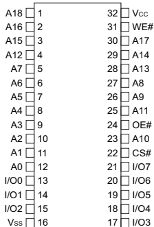
32 DIP 32 CSOJ 32 Flatpack Top View
